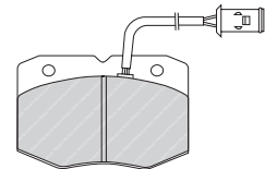
FVR1315 BRE 29121 165 x 66 x 18mm
