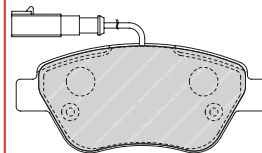
FDB1556 TRW 20261 146.6 x 59.8 x 19.4mm
