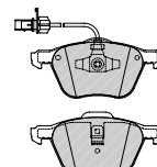
FVR1497 ATE 23269 161 x 72.9/74.4 x 20.1mm
