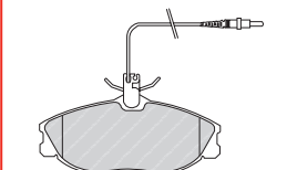
FDB1168 ATE 21430 142 x 47.5 x 17mm
