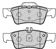
FDB1526 ATE 23334 141 x 59.5 x 15.8mm
