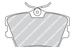
FVR1518 ATE 21883 156 x 68.5 x 19.6mm
