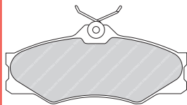
FVR1132 LUC 21882 95 x 57.3 x 17.3mm
