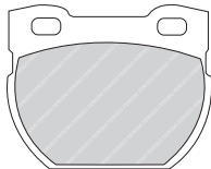
FDB1994 LKD 23471 88.5 x 68.8 x 17.8mm
