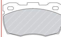
FDB1615 TRW 24191 162.6 x 58 x 18mm
