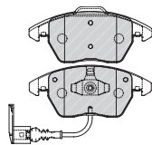
FVR785 LUC 20124 130 x 54.5 x 19mm
