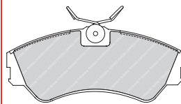
FVR1484 ATE 23034 157 x 78.9 x 18.9mm
