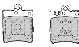
FDB1322 ATE 21898 64 x 78 x 15.5mm
