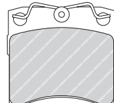
FVR1163 ATE 21883 156 x 68.5 x 19.6mm
