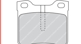
FVR1778 BRE 29192 163.2 x 66.9 x 20.8mm
