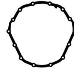
RDS 55473 13-3/4" X 13-1/4" 14-Holes
