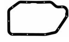
TOS 18660 16-3/8" X 9-7/16" 10-Holes
